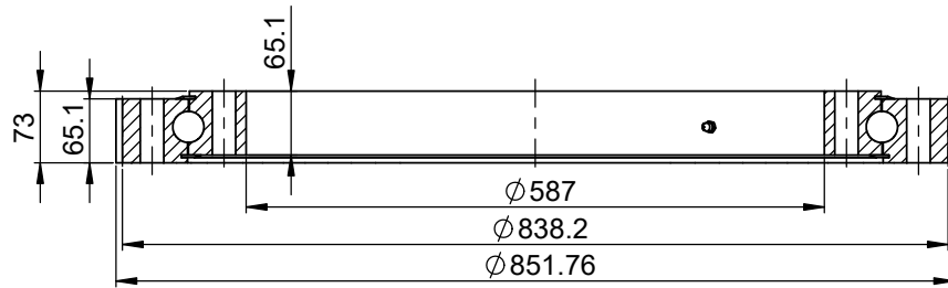
VIEW F-F
