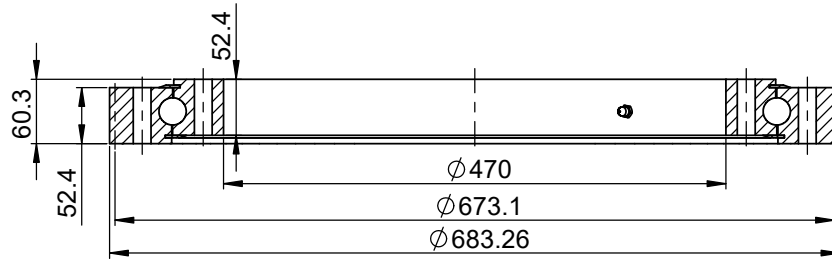
VIEW F-F
