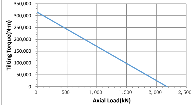
Tilting Torque VS Axial Load
